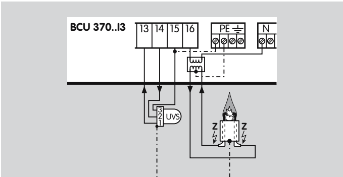
BCU 370..I3 for 120 V, ignition by electrode to electrode with centre tap for secondary earthing
