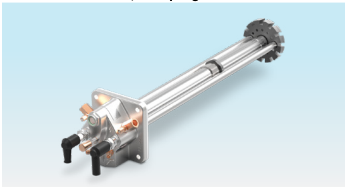
Burner insert BIO with purged electrodes
