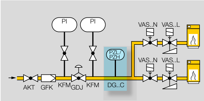
The DG..C controls the minimum or maximum gas inlet pressure on high-performance boilers.
